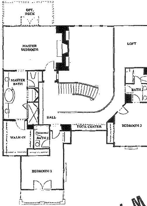
LEVEL 2
